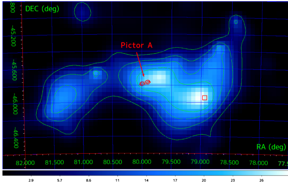
Figure 2. Fermi -LAT TS map ( >200 MeV) centered on Pictor A, showing the presence of multiple \gamma -ray peaks in the field. Contamination from nearby sources are modeled as part of the background that also includes Galactic/extragalactic diffuse \gamma -ray emission. The green contours correspond to TS values of 5, 10, 15, and 20, while the red contours indicate 1.4 GHz radio emission from Pictor A (Perley et al. 1997). The position of a blazar, BZQ J0515–4556, is also shown as red box. The peak near the center of the map (TS = 20) is almost exactly coincident with the position of Pictor A. The TS peaks associated with Pictor A and with BZQ J0515–4556 are only marginally resolved. The TS value quoted here and in Table 2 for Pictor A was evaluated using a source model that included point sources at the position of BZQ J0515–4556 and at R.A. = 81^{\circ}35' , decl. = -45^{\circ}78' .
